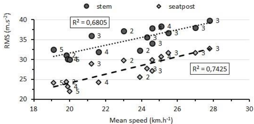
Figure 2. Linear relationship between RMS value and mean speed.
