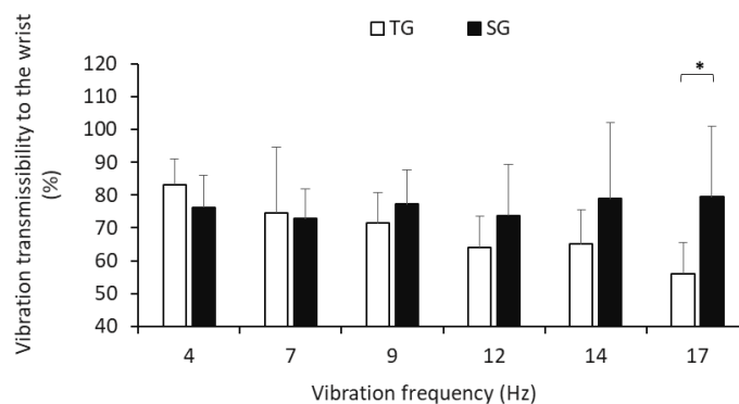
Figure 2. Comparison of transmissibility of vertical acceleration from the ergometer to the wrist with traditional grips (TG) and SPIRGRIPS® (SG)
